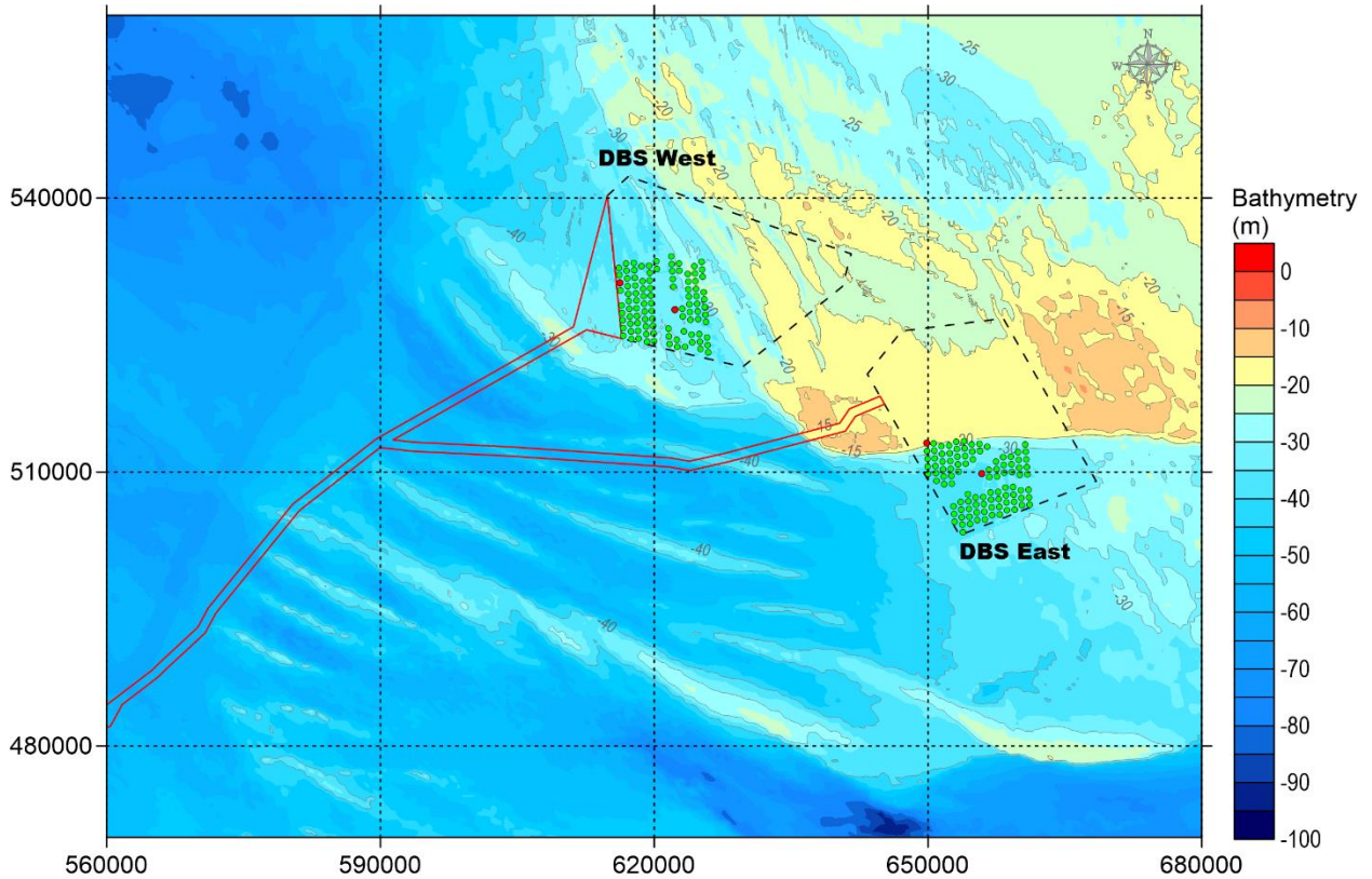
Figure 8-3-11: Windfarm Layout for Option 2 (indicative alignment of turbines spaced closer together) (red dots: platform foundations 15m diameter)
