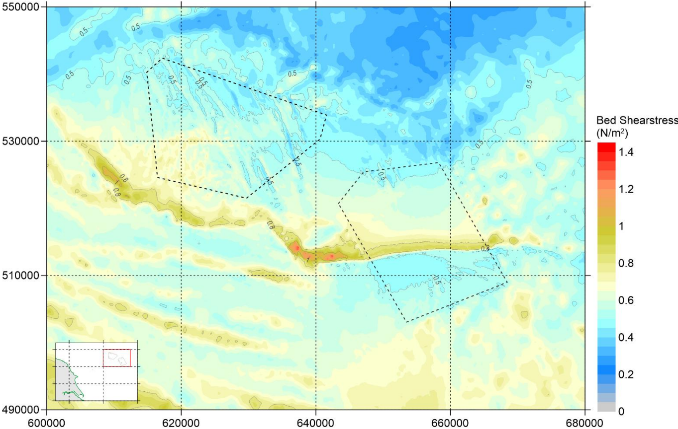
Figure C-31: Maximum Bed shear Stress Over 30 Days- Baseline
